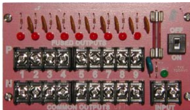
PDM-9G5-P1.1 shown
